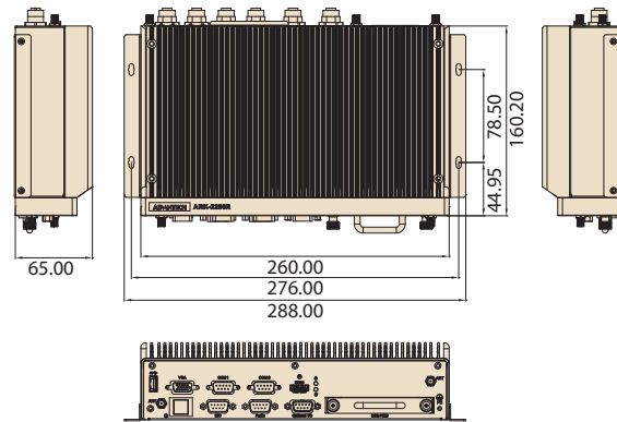
ARK-2250R
